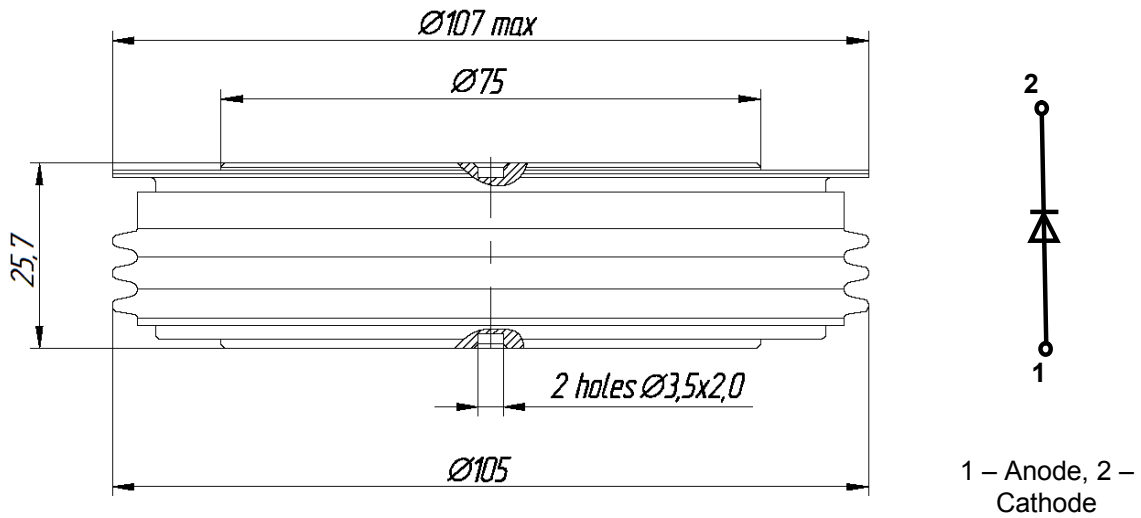
Fig. 1. Device Outline Drawing (dimensions in mm)
